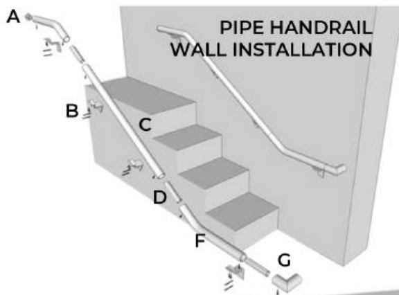
G. 90° Pipe Handrail Return Kit
