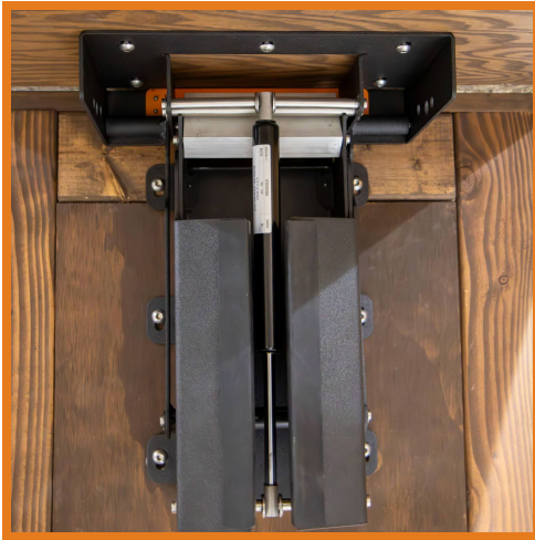
Drop Gate Hinge Mechanism
