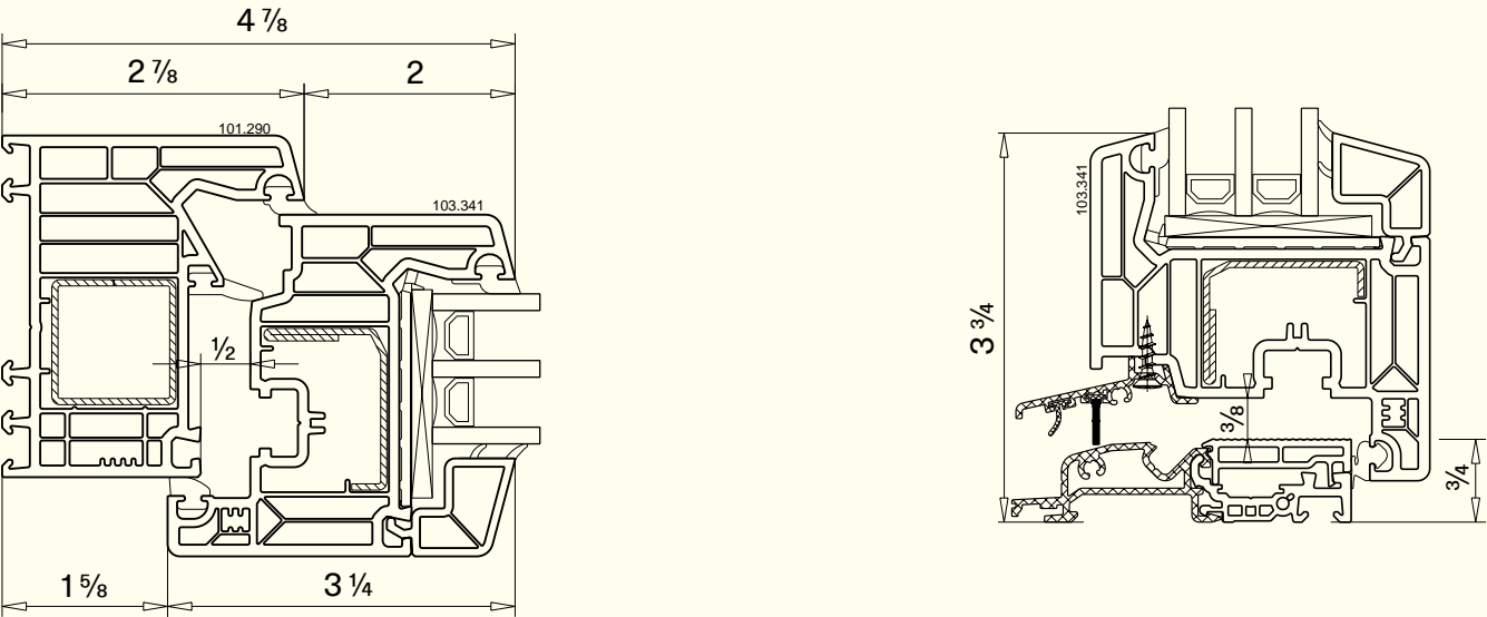
OptiPro Triple Gasket Window
