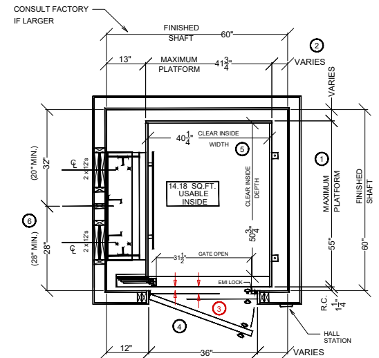
STANDARD HOISTWAY PLAN
