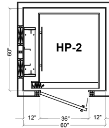
HP-2: Left-hand rail placement
