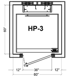
HP-3: Rear rail placement (not available with Pitless)
