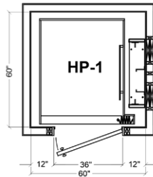
HP-1: Right-hand rail placement
