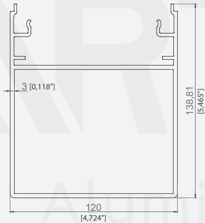
YAN KAYIT PROFİLİ / SIDE BEAM PROFILE
