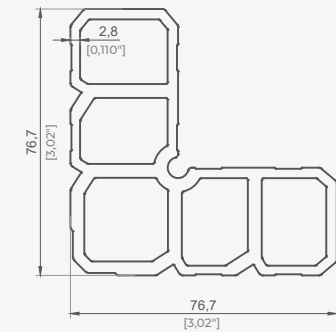
Cam Panel Köşe Takoza Profili / Glass Panel Corner Block Profile
