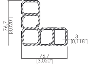
Cam Panel Köşe Takozu Glass Panel Corner Block Profile
