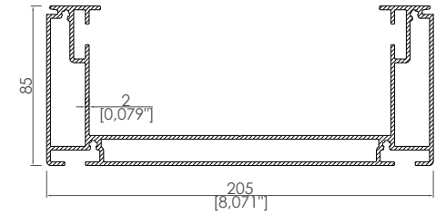
Dere Profili Gutter Profile
