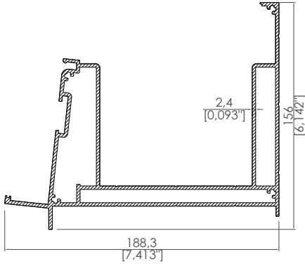
188,3x156 Düz Dere 188,3x156 Gutter Profile
