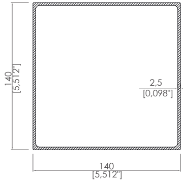
140x140 Dikme Profili 140x140 Pillar Profile
