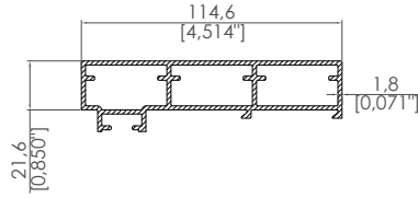
Yan Ray Profili Side Rail Profile
