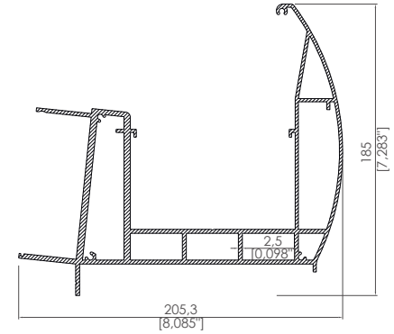
205,3x185 Oval Dere Profili 205,3x185 Oval Gutter Profile
