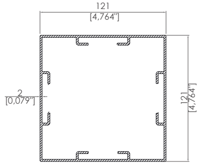
Direk Ayak Profili Pillar Profile
