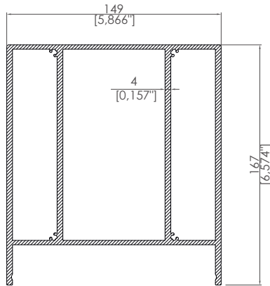
Orta Destek Profili Middle Support Profile
