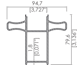
Kulplu Panel Profili Glass Panel Handle Profile
