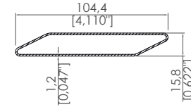
104,4x15,8 Panel Profili 104,4x15,8 Panel Profile
