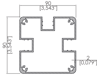
Standart Dikme Profili Standart Pillar Profile
