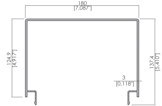
Dikme Kapak Profili Pillar Cover Profile
