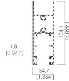
Cam Panel Alt ve Üst Profili Glass Panel Top and Bottom Profile
