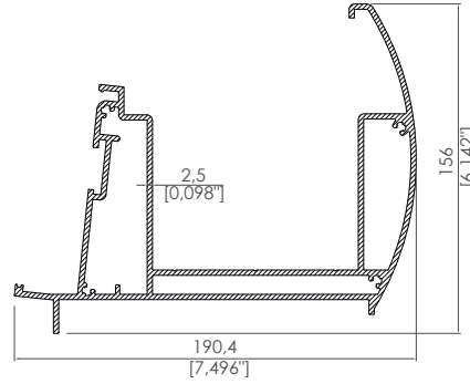
190,4x156 Oval Dere Profili 190,4x156 Oval Gutter
