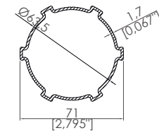
Motor Borusu Eki Motor Tube Connection
