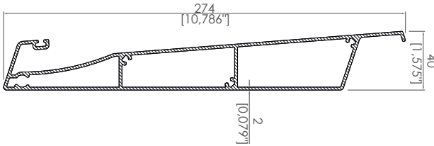
Panel Profili Panel Profile
