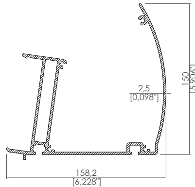
158,2x150 Oval Dere 158,2x150 Oval Gutter
