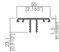
Orta Cam Kapak Profili Middle Glass Cover Profile
