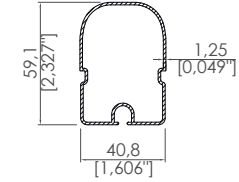
40,8x59,1 Kumaş Profili 40,8x59,1 Fabric Support Profile
