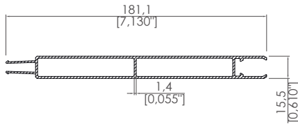
180x15 Panel Profili 180x15 Panel Profile
