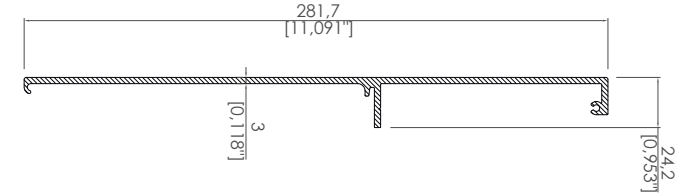
Dere Kapak Profili Gutter Cover Profile
