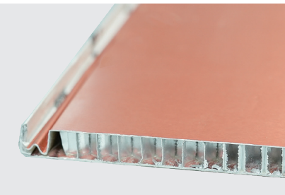
蜂窝芯 Honeycomb Core
