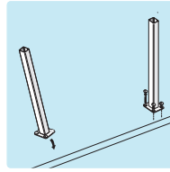
Install Posts
