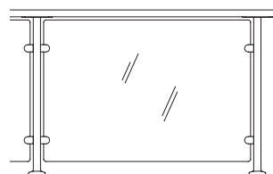
36" SPECTRUM GLASS WITH FLAT GLASS PANEL CONNECTORS
