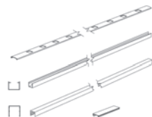
Top and Bottoms Rails - Glass (glass insert, rubber blocks, and support leg included)
