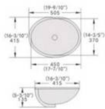
Cutaway View
